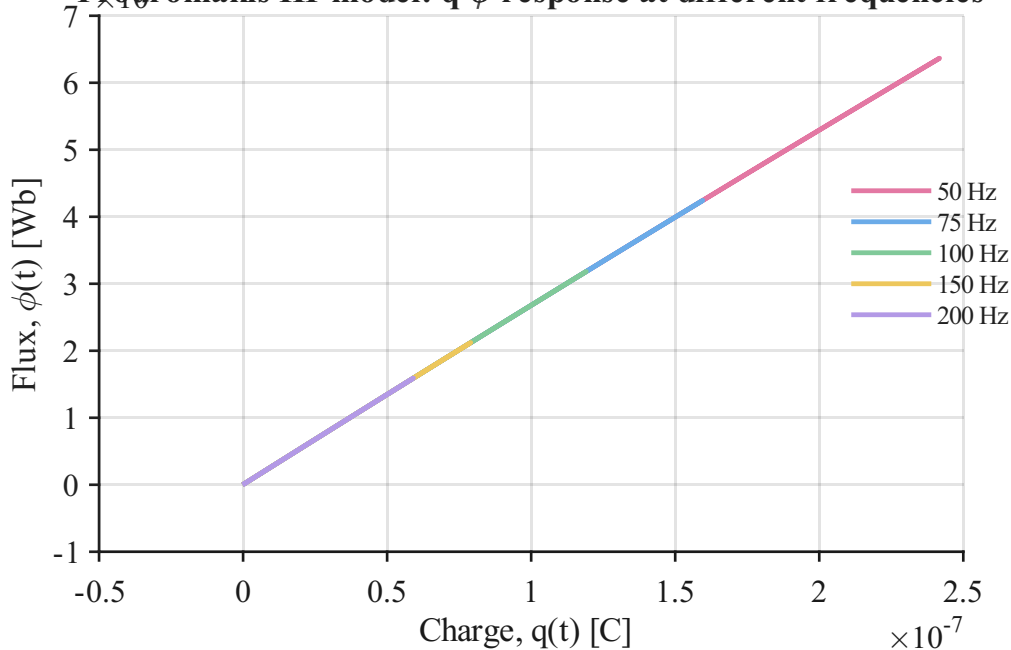
Prodromakis HP model: q - \phi response at different frequencies
