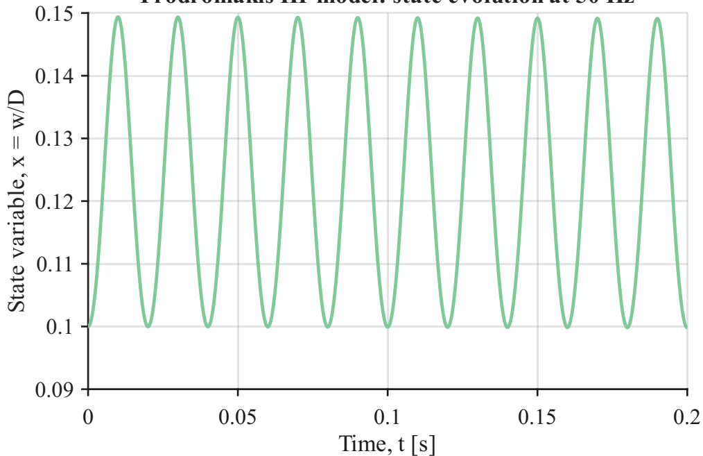
Prodromakis HP model: state evolution at 50 Hz
