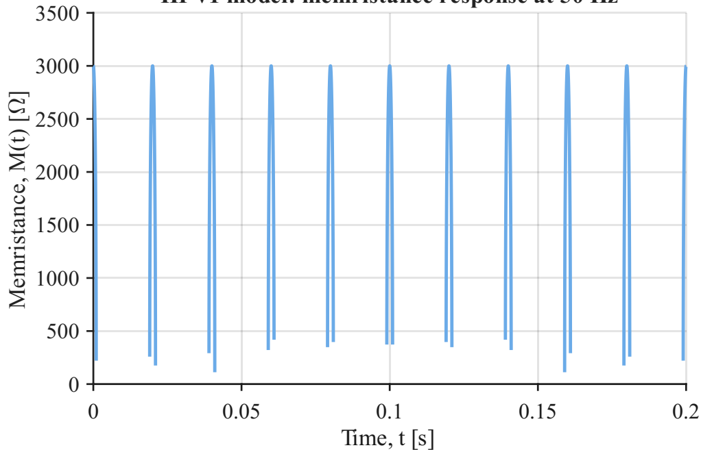
HP v1 model: memristance response at 50 Hz
