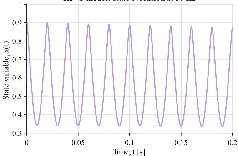
HP v3 model: state evolution at 50 Hz
