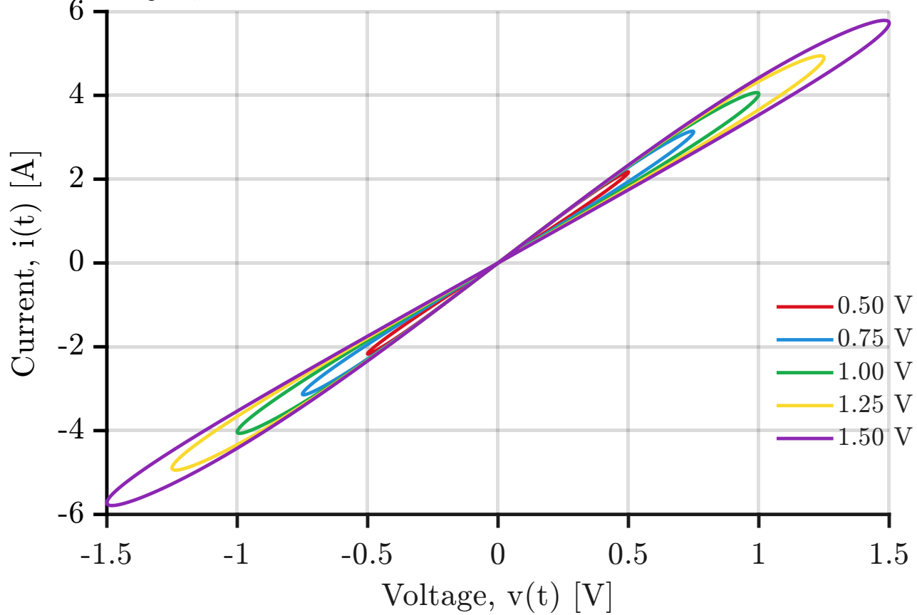
HP-105 Joglekar model: I-V response at different amplitudes
