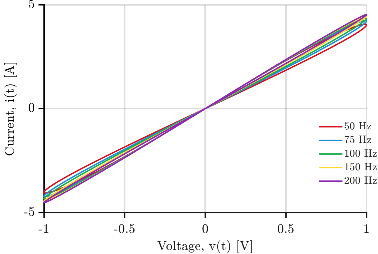
HP1050 model: I-V response at different frequencies
