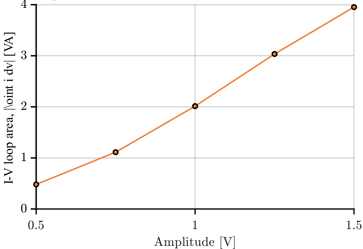
HP-10 Doglekar model: hysteresis area versus amplitude
