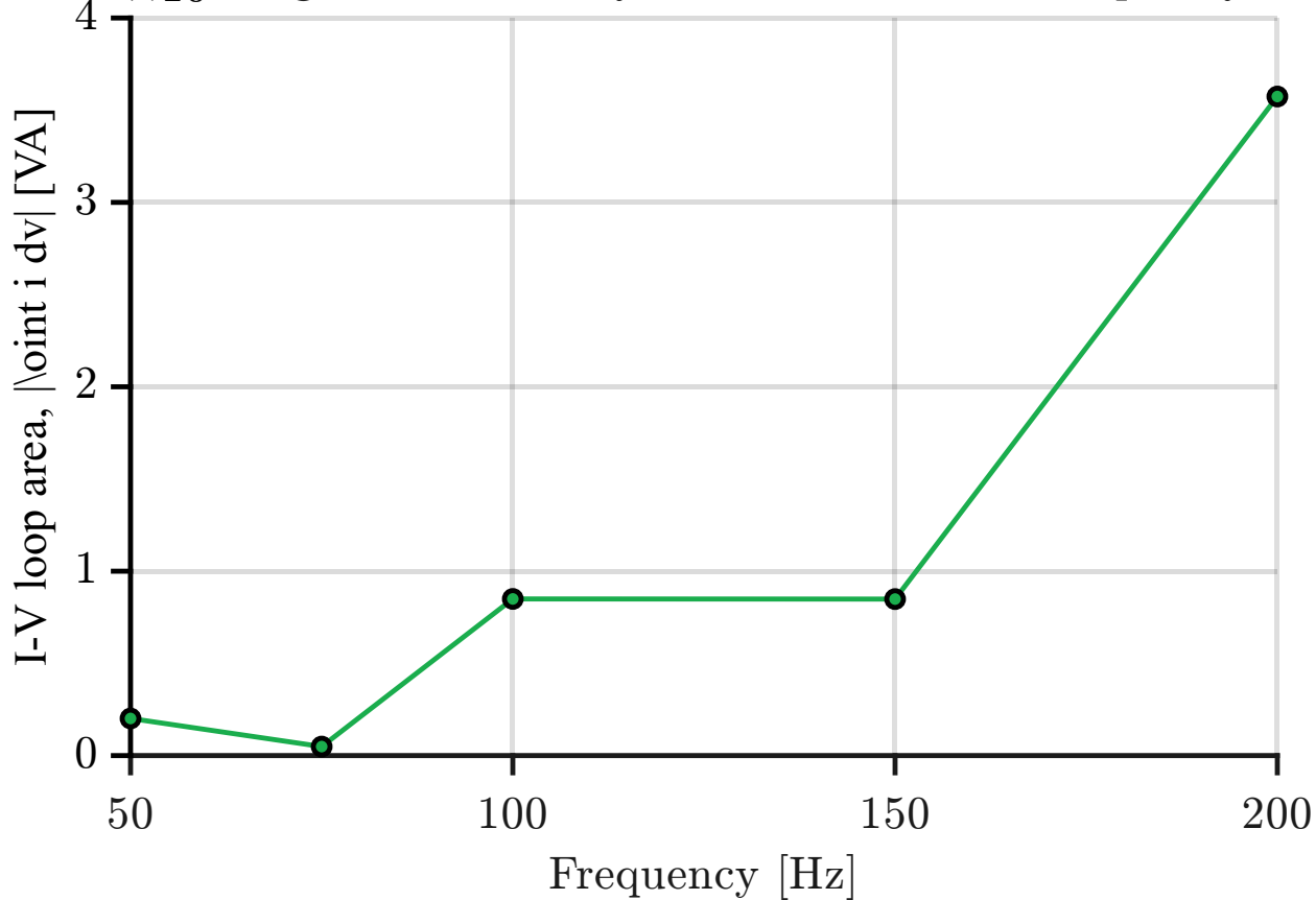
HP Joglekar model: hysteresis area versus frequency
