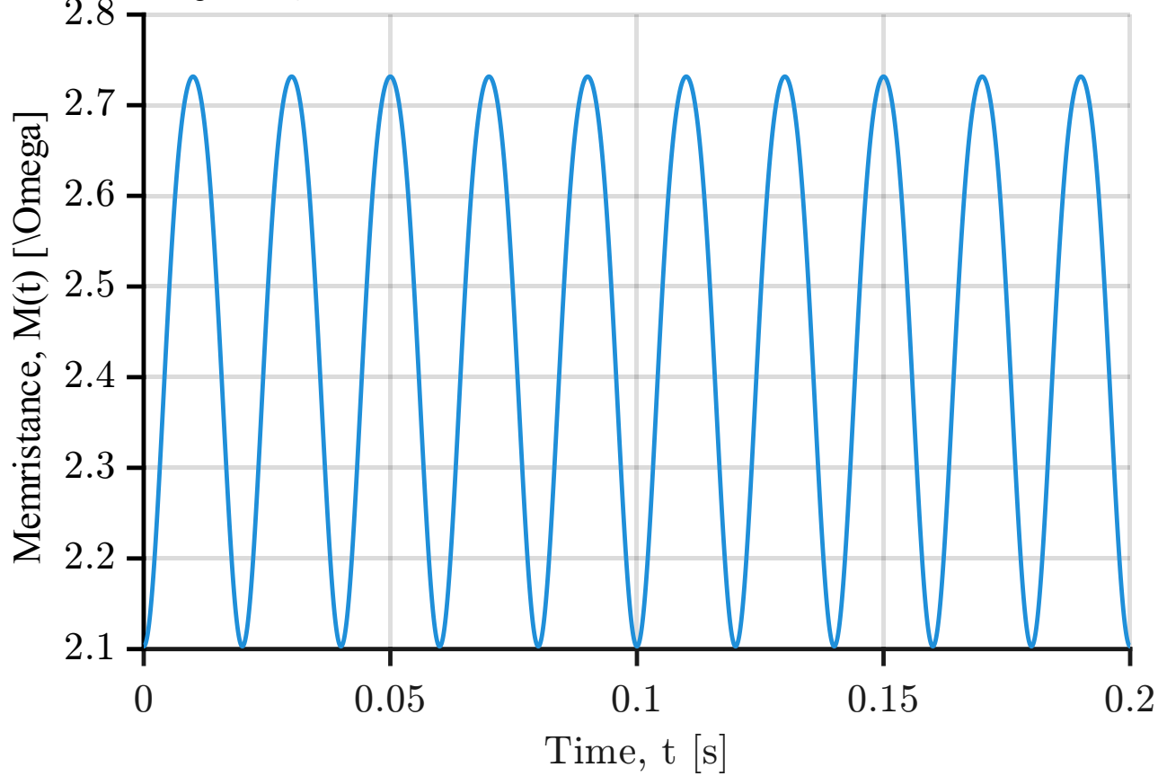
HP Joglekar model: memristance response at 50 Hz
