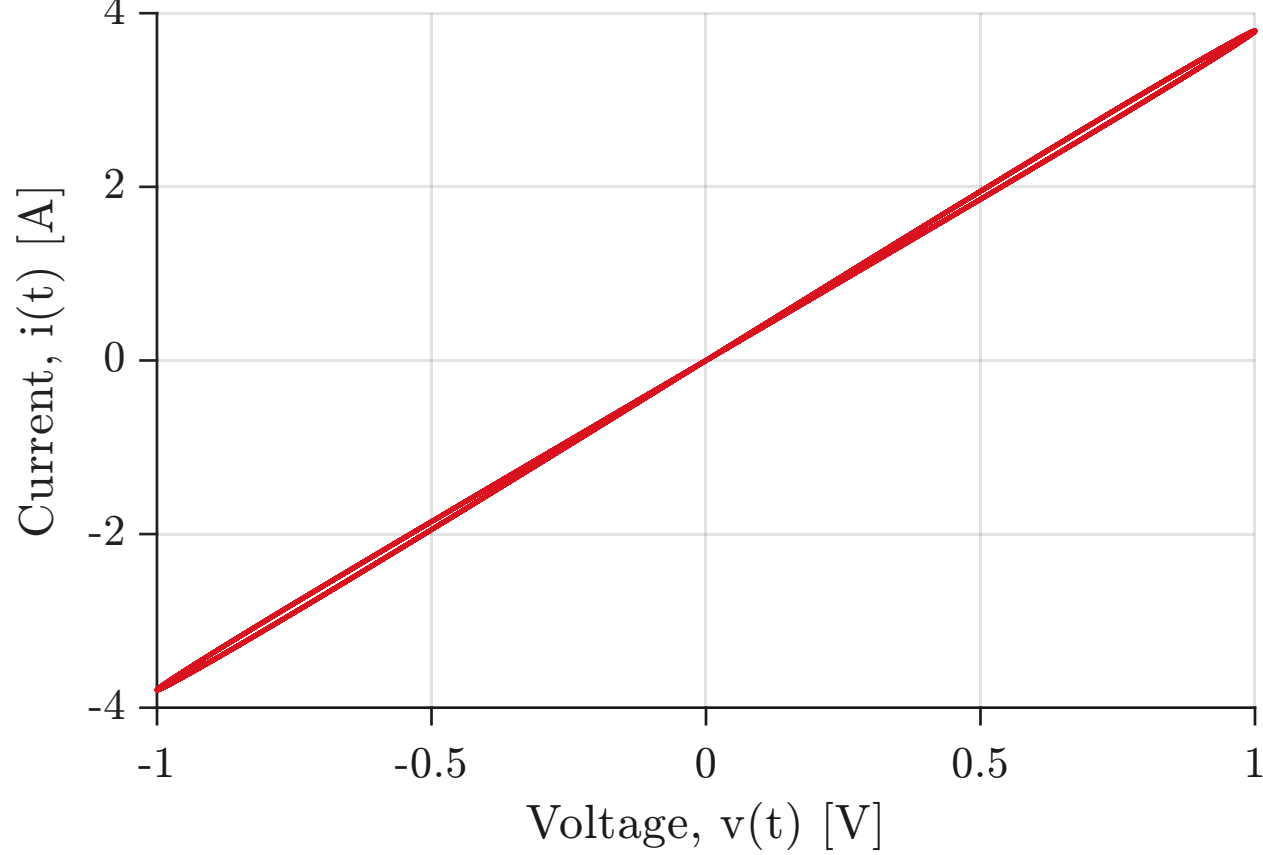
Prodromakis HP model: I-V response at 50 Hz
