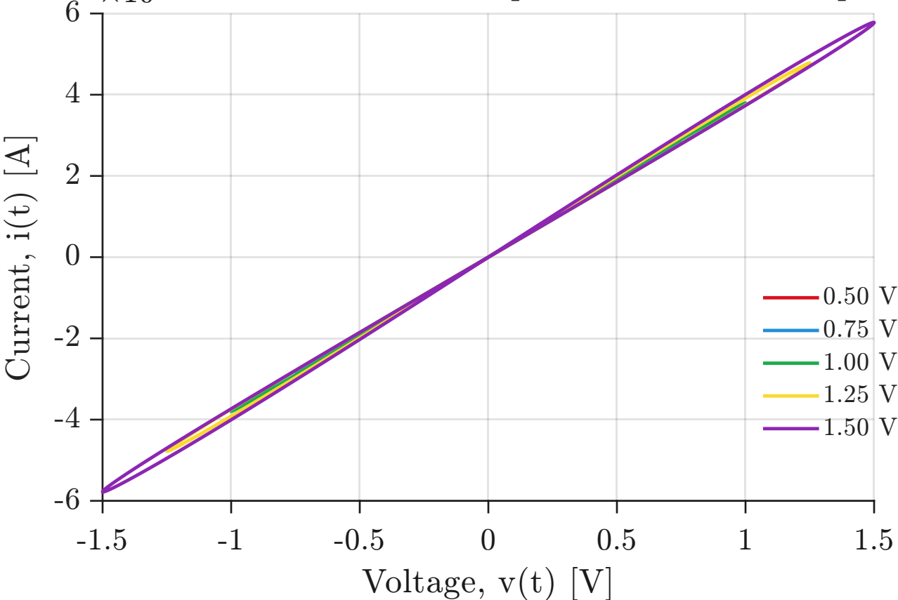
Prodromakis HP model: I-V response at different amplitudes
