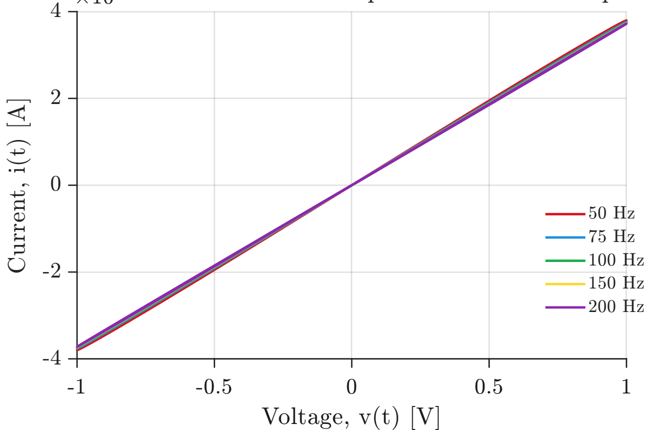
Prodromakis HP model: I-V response at different frequencies
