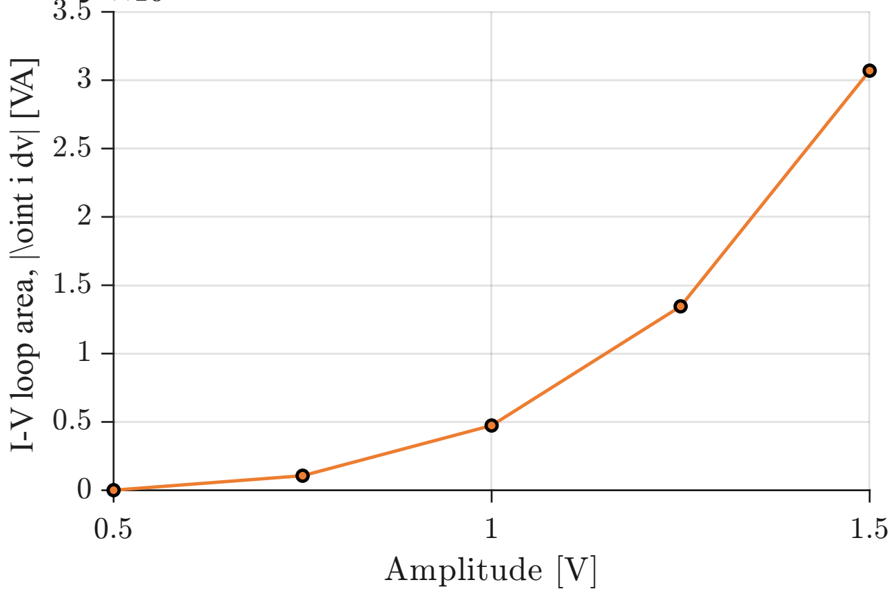
Prodromakis HP model: hysteresis area versus amplitude
