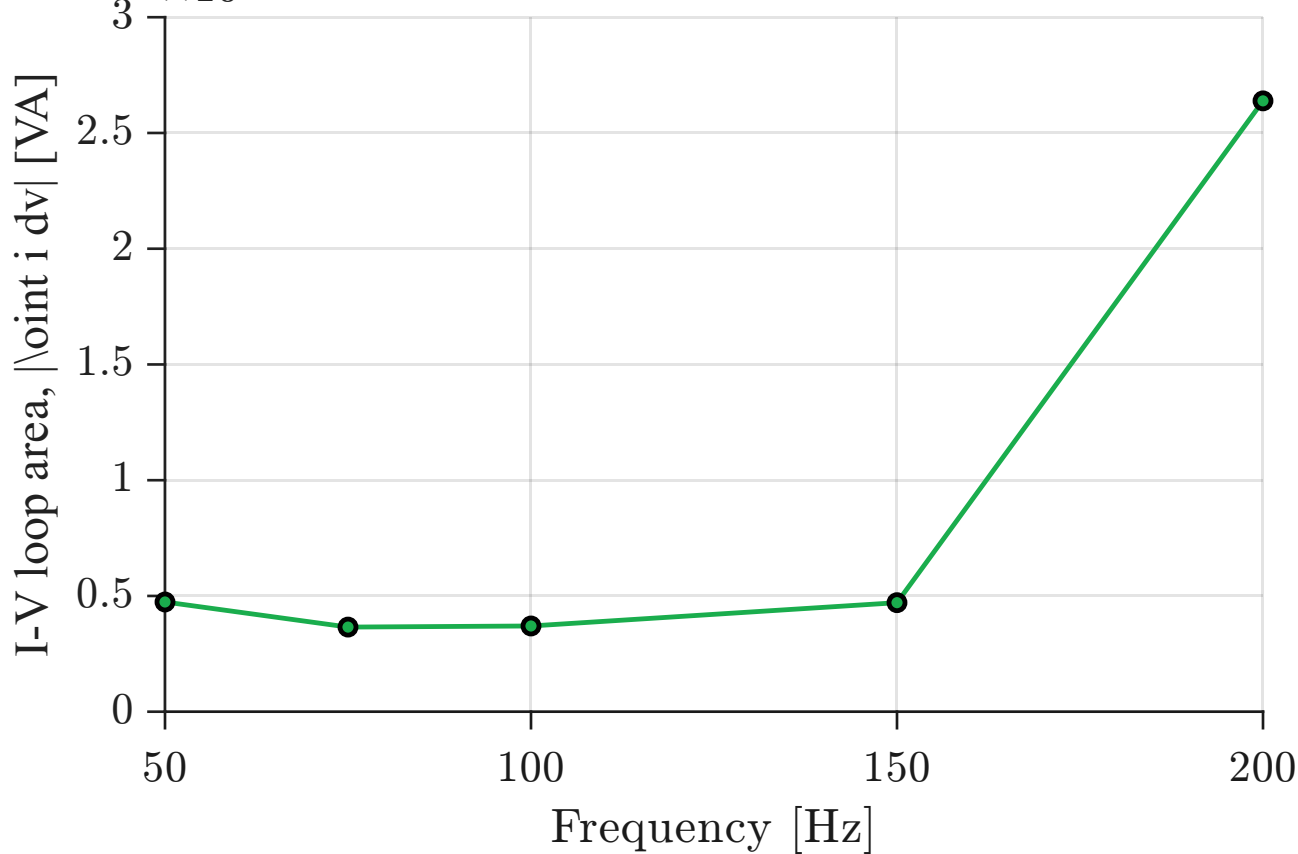
Prodromakis HP model: hysteresis area versus frequency
