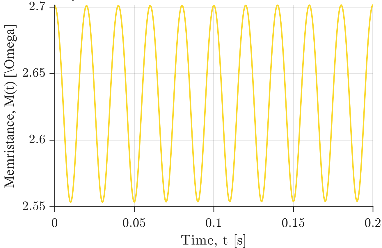
Prodromakis HP model: memristance response at 50 Hz
