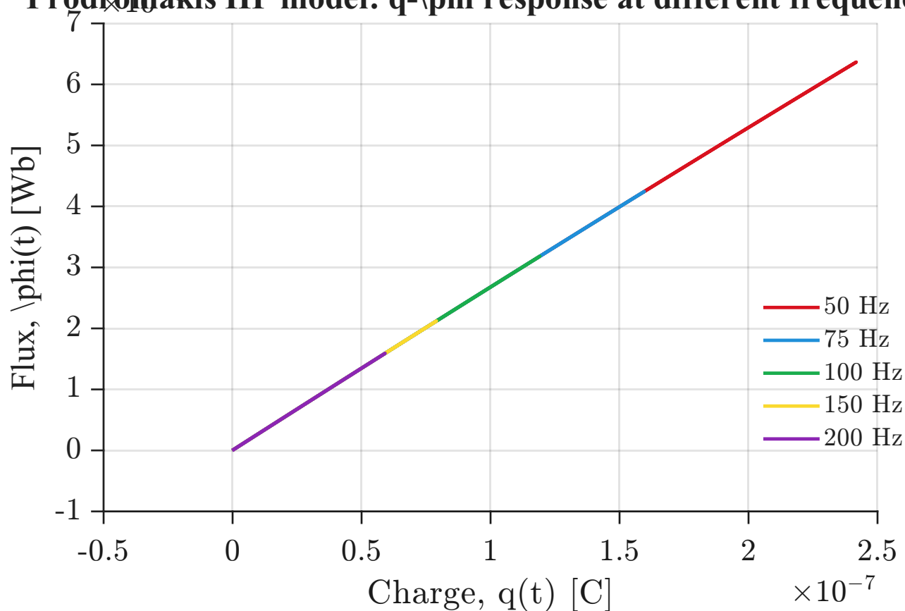
Prodromakis HP model: q - \phi response at different frequencies
