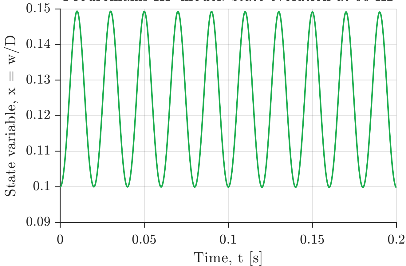
Prodromakis HP model: state evolution at 50 Hz
