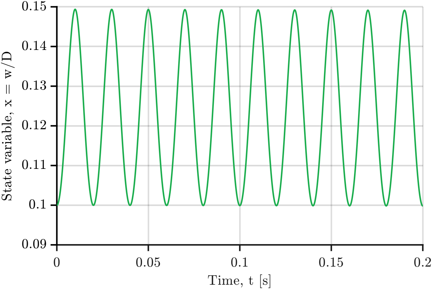
Prodromakis HP model: state evolution at 50 Hz
