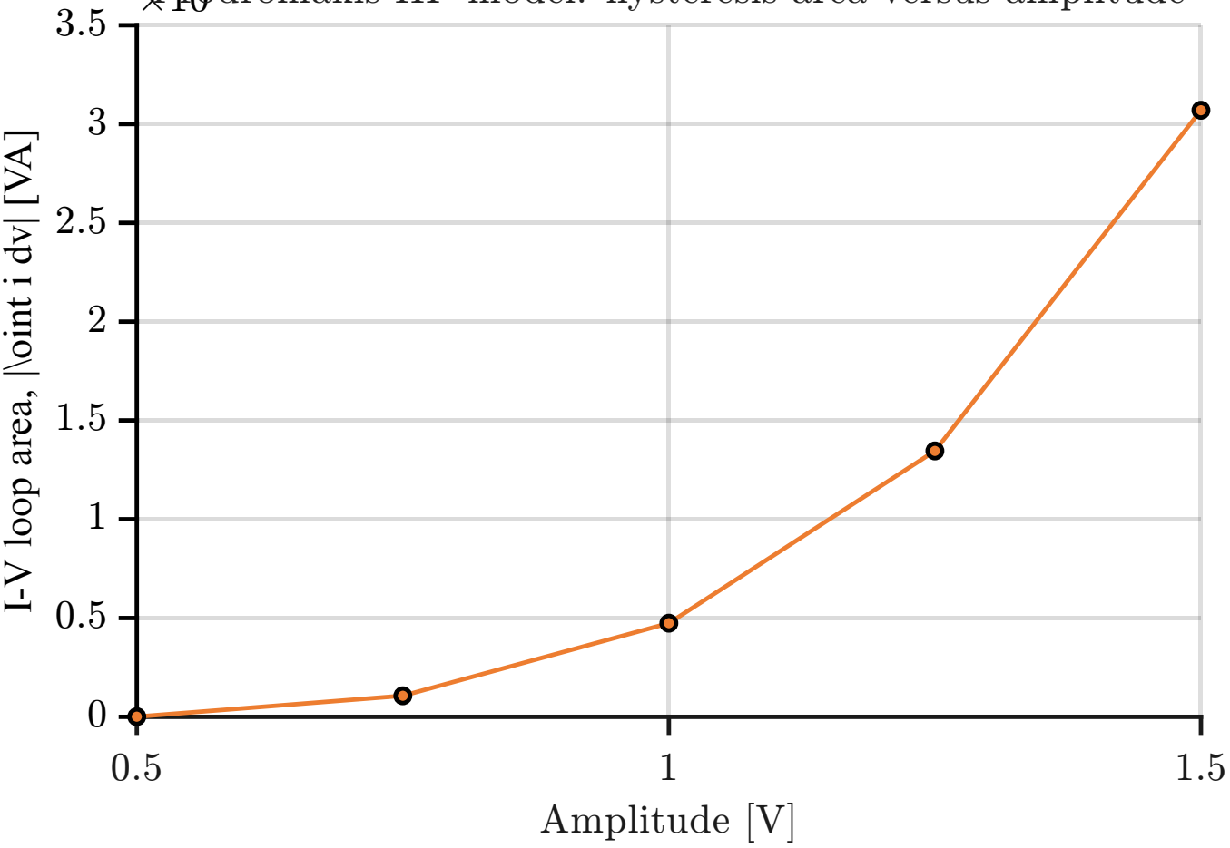
Figure 10: Pindromakis HP model: hysteresis area versus amplitude
