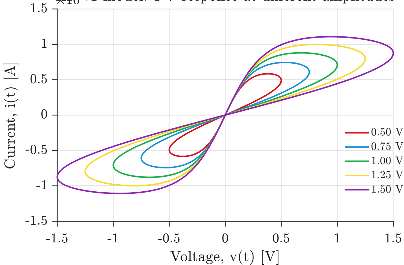
HP-10-v1 model: I-V response at different amplitudes
