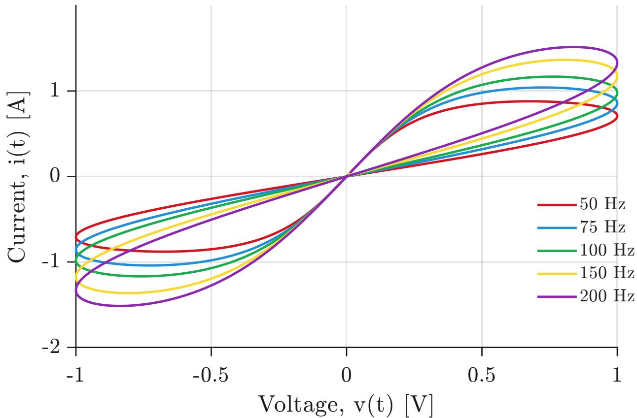
HP10-v1 model: I-V response at different frequencies
