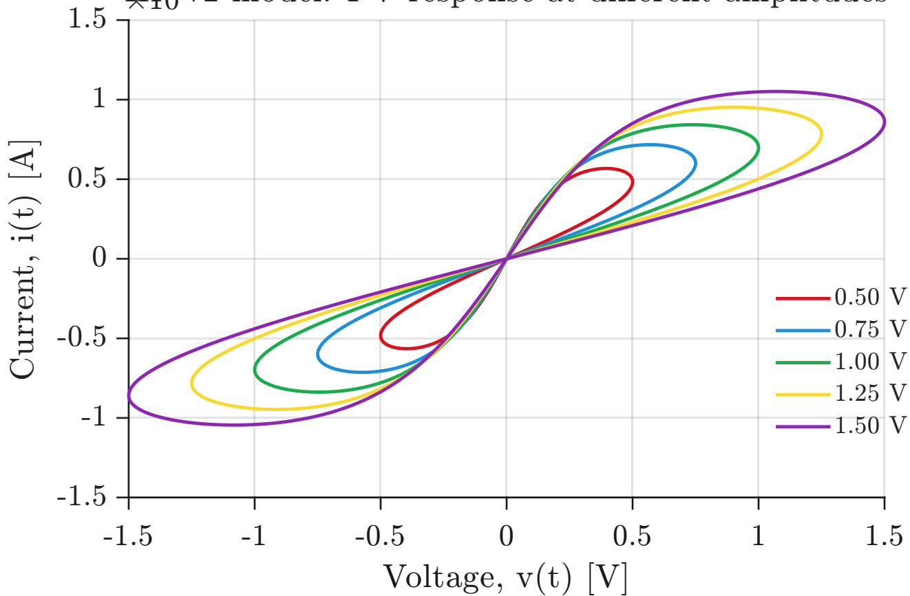
HP-10-v2 model: I-V response at different amplitudes
