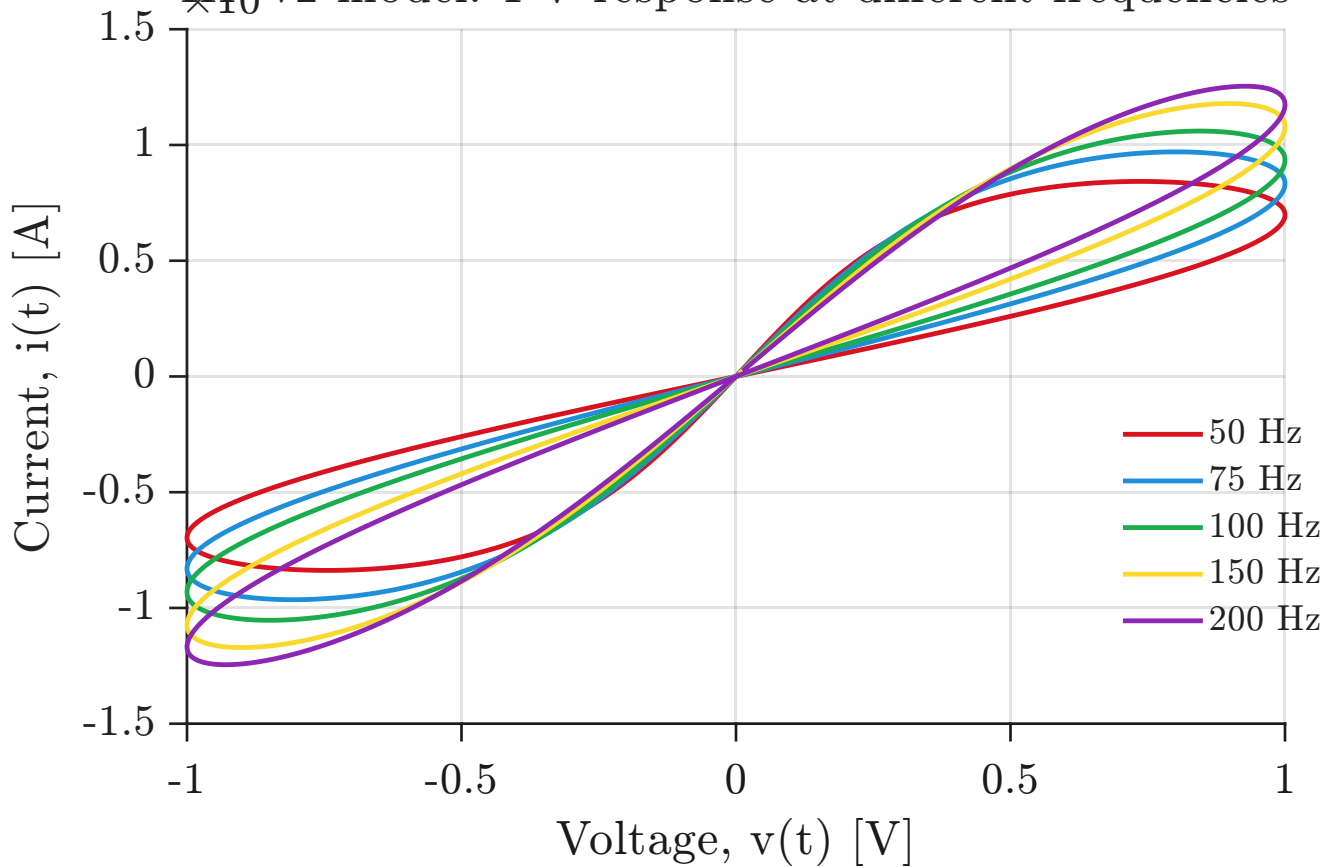
HP-10-v2 model: I-V response at different frequencies
