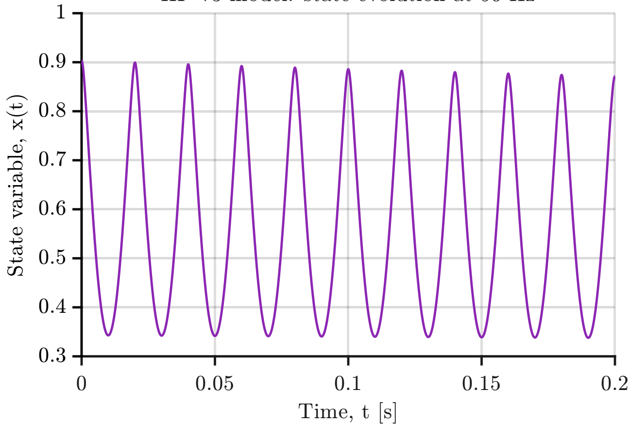
HP v3 model: state evolution at 50 Hz
