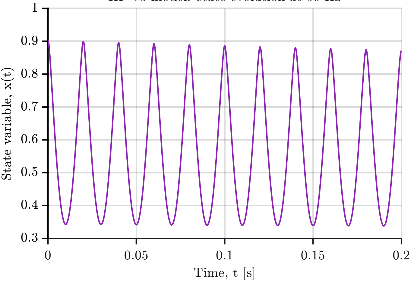
HP v3 model: state evolution at 50 Hz
