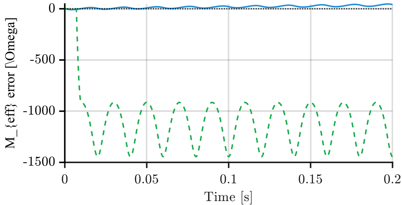
Effective memristance error
