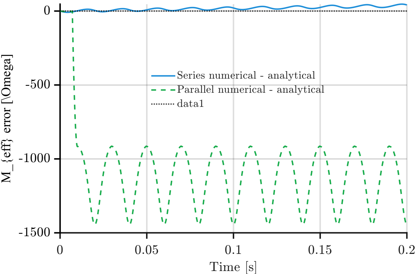
Effective memristance error
