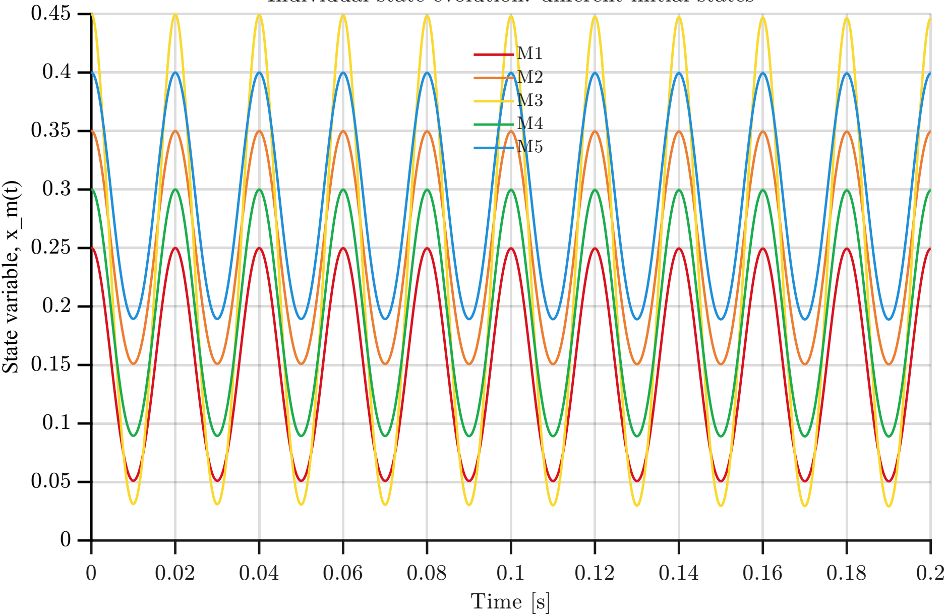
Individual state evolution: different initial states
