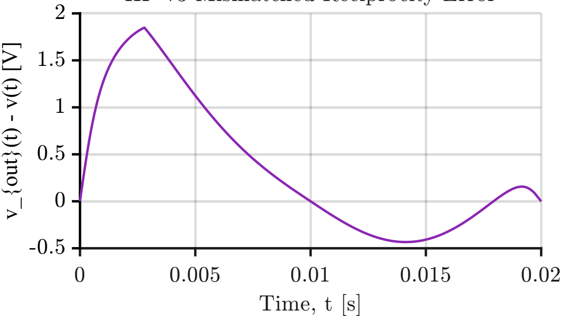
HP v3 Mismatched Reciprocity Error
