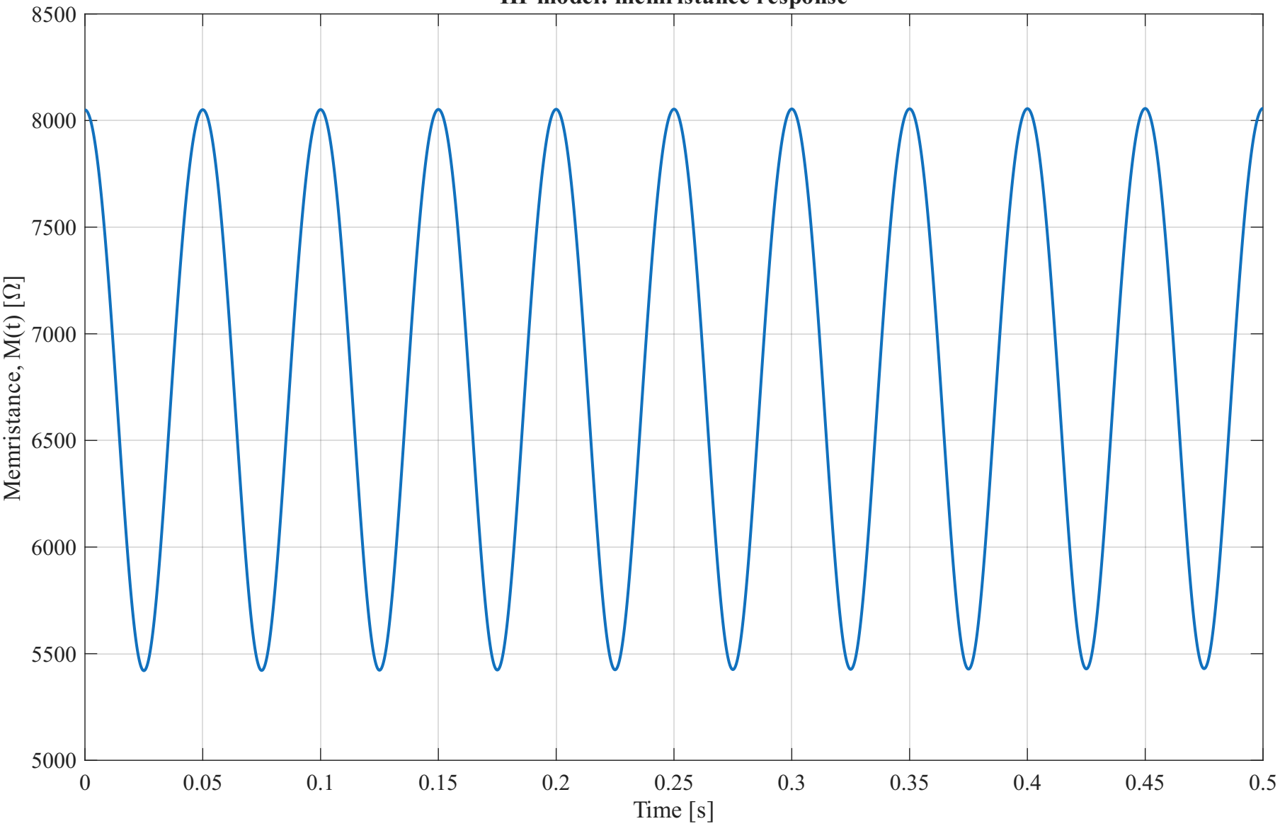
HP model: memristance response
