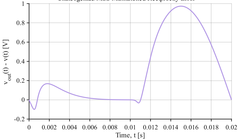
Chalcogenide/MSS Mismatched Reciprocity Error
