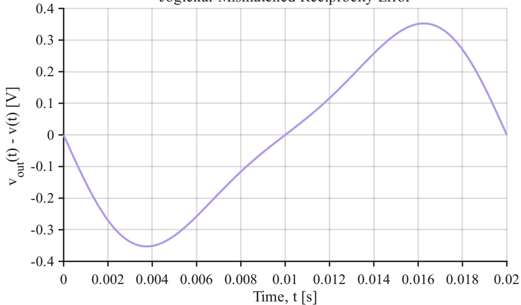
Joglekar Mismatched Reciprocity Error
