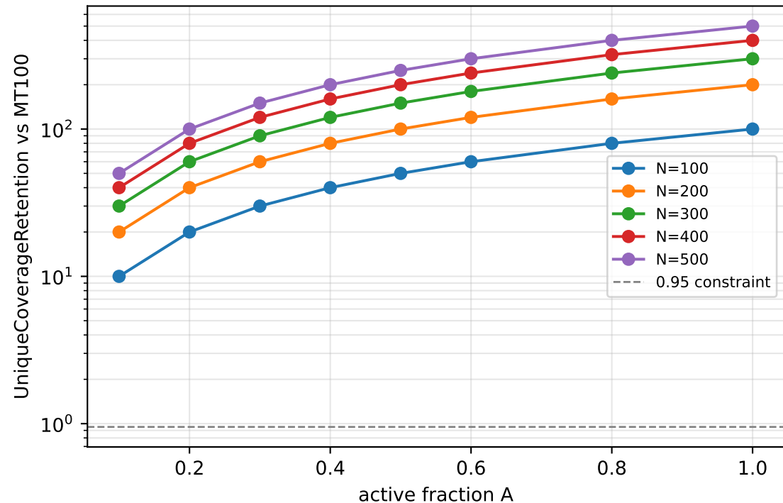
PoCol exceeds MT100 unique coverage k-fold at every fraction
