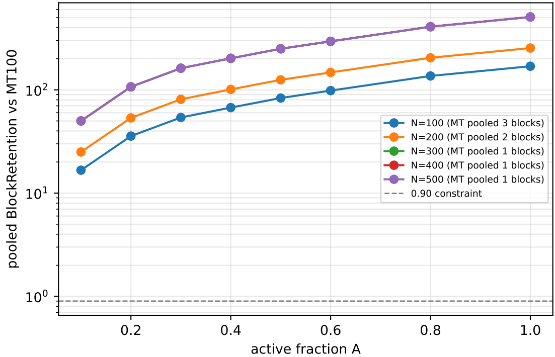
PoCol out-produces the same-template control at every fraction (sparse MT100 denominators shown)
