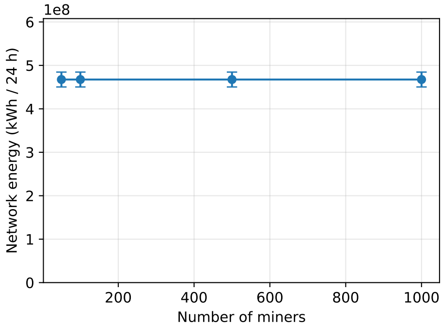
(a) Total PoW energy is invariant to miner count
