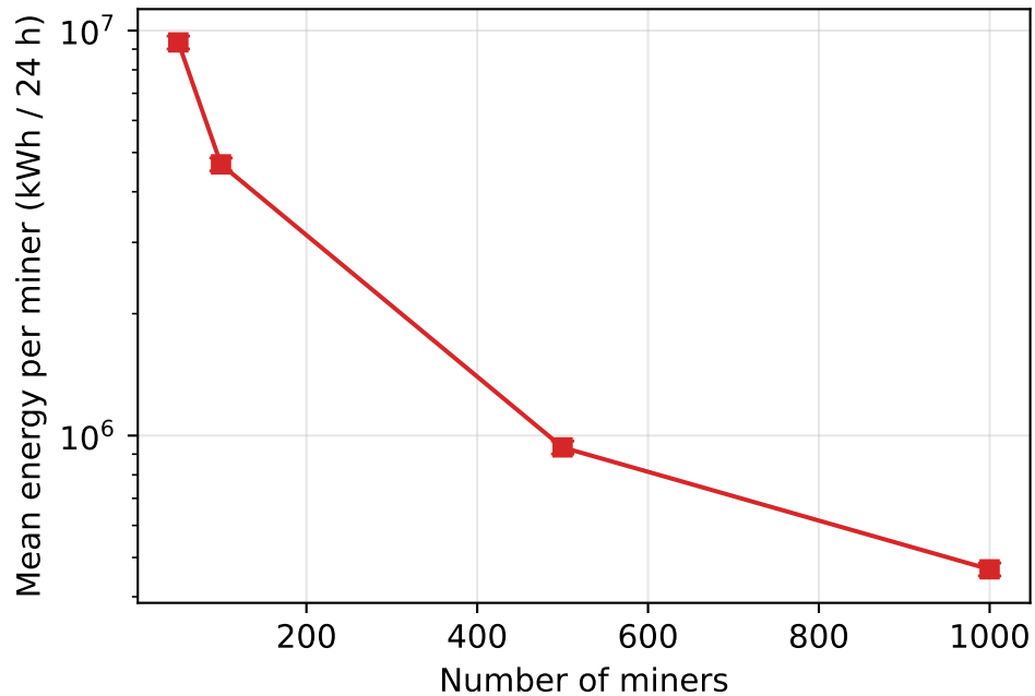
(b) Per-miner energy falls \sim 1/N
