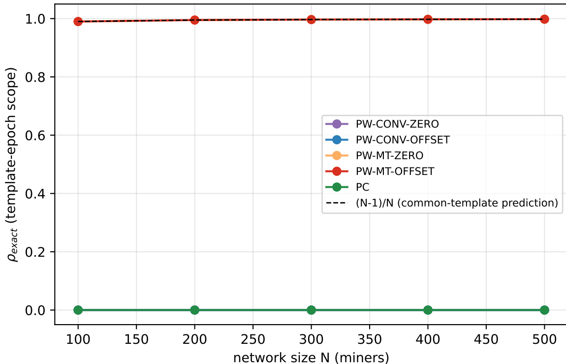
Exact-input duplication: zero for CONV and PC; (N-1)/N for the common-template comparator
