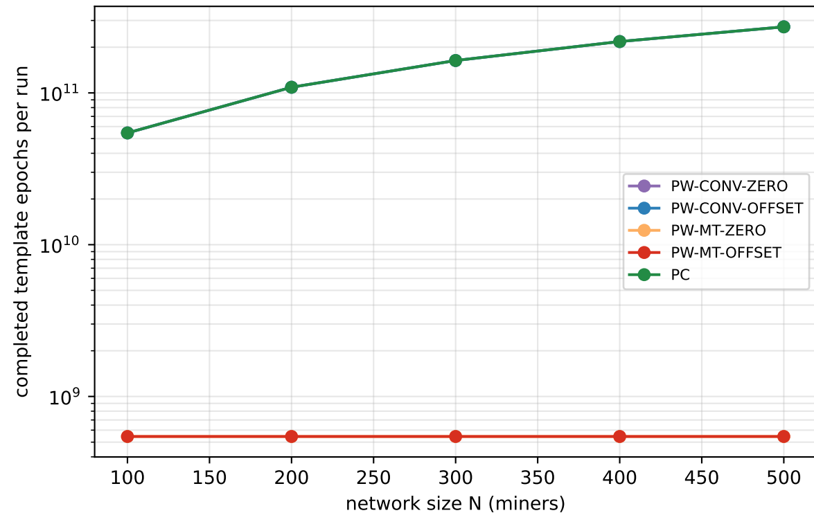
Extranonce-induced template renewal: per-miner epochs for CONV/PC ( N \times 5.45e8 ), network epochs for MT ( 5.45e8 )
