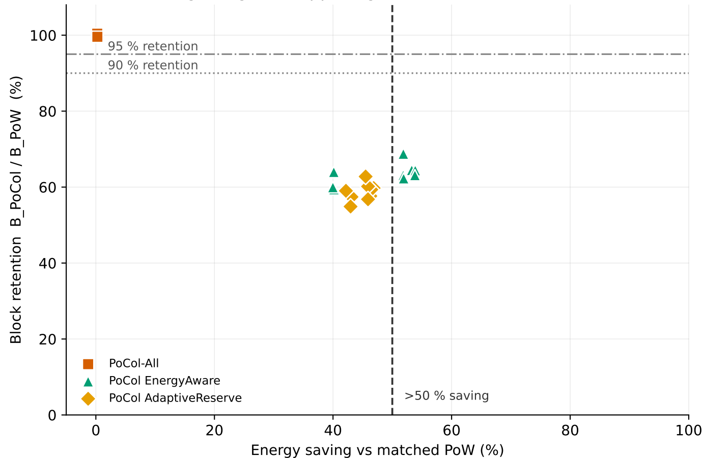
Energy saving vs block retention (alpha_0) target region is upper right of both reference lines
