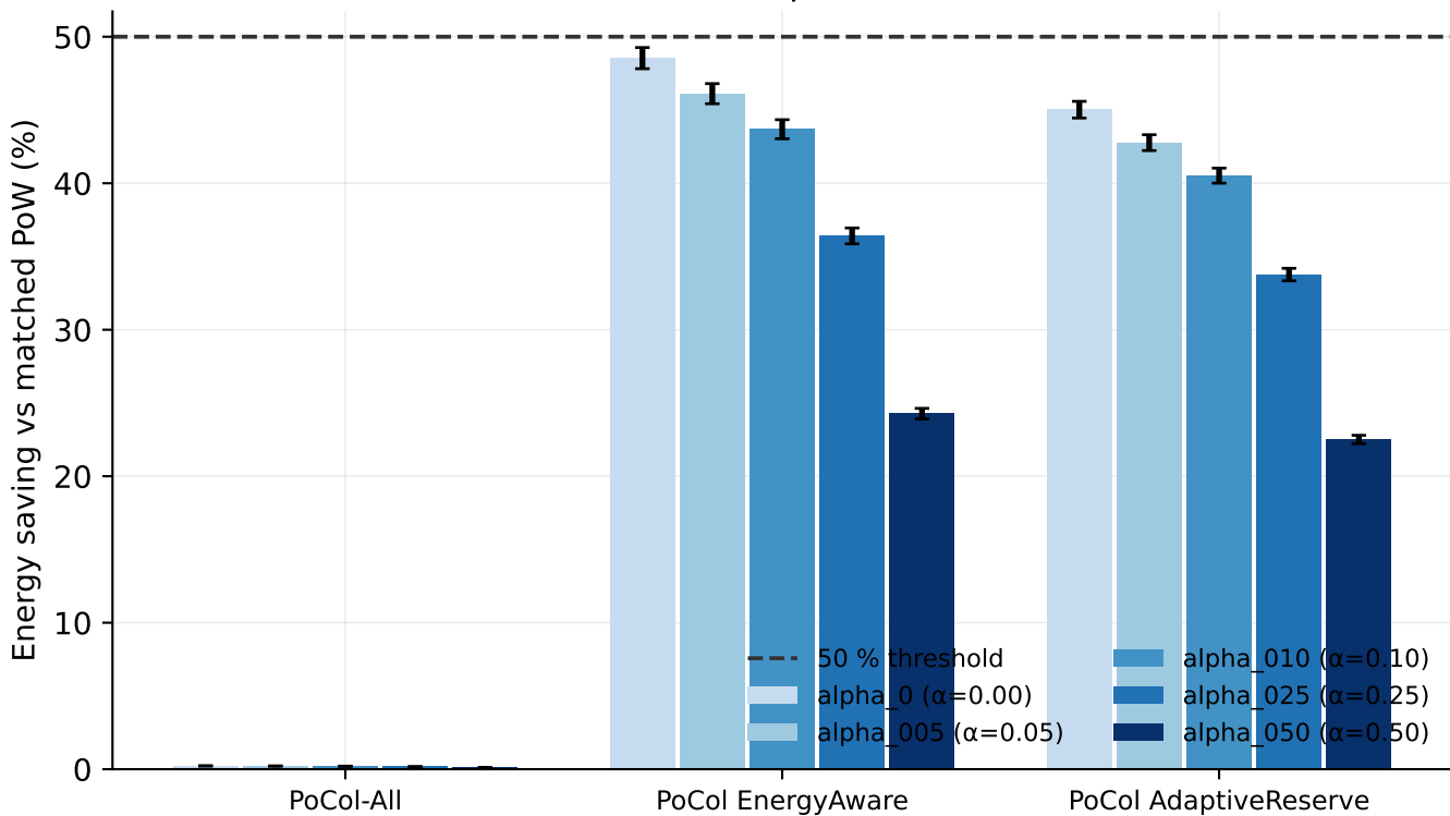
Energy saving by PoCol policy and low-power assumption ( \alpha values are model assumptions, not vendor modes)
