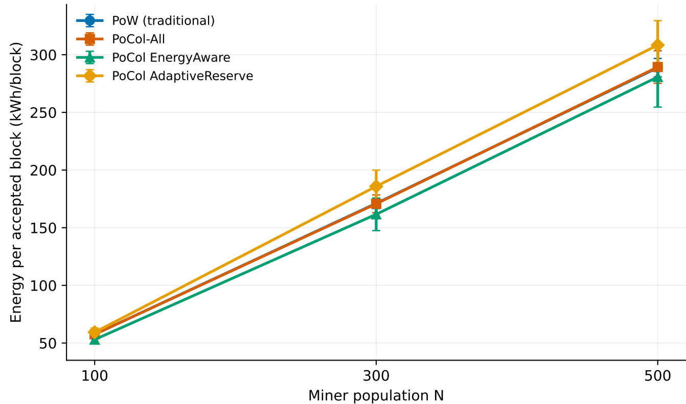
Energy per accepted block ( \alpha = 0.10 )
