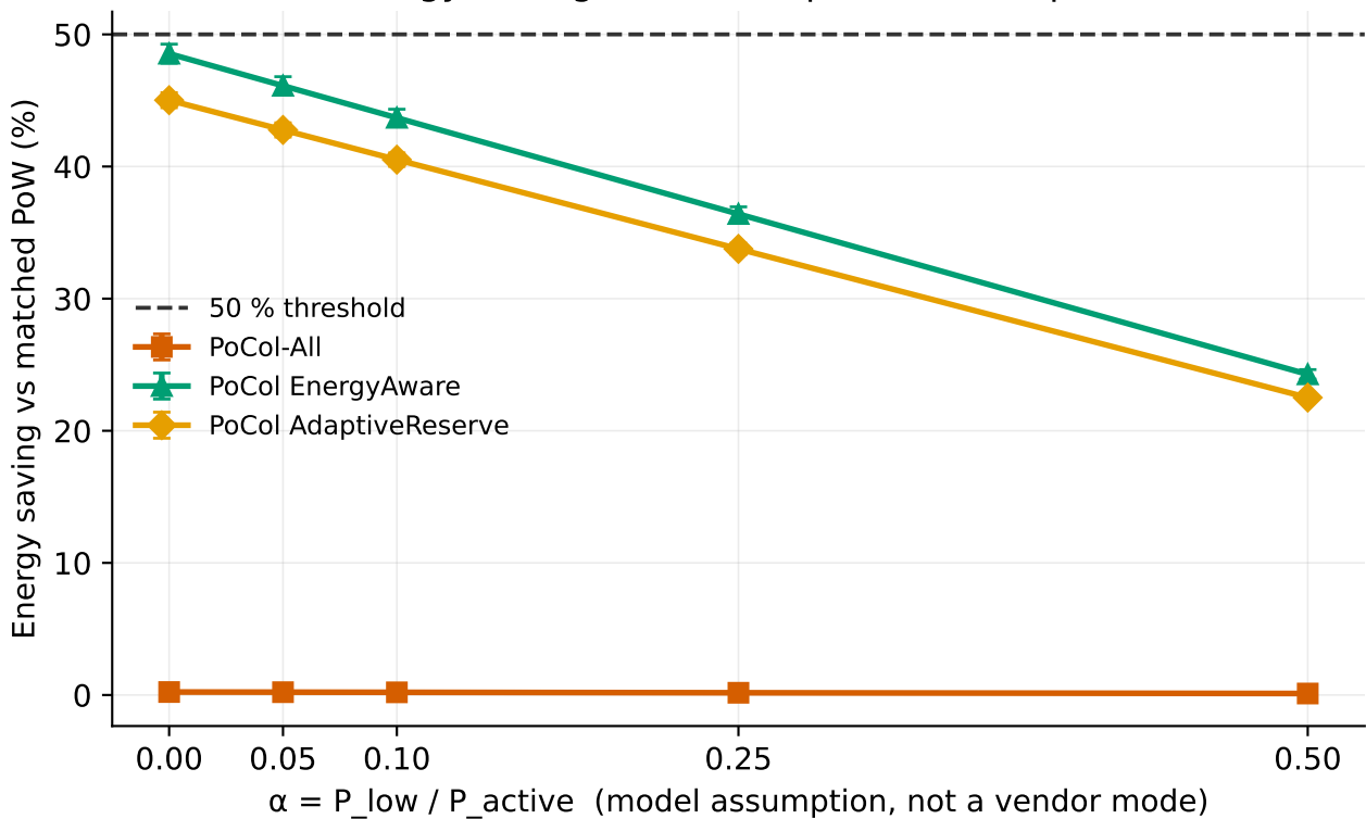
Energy saving vs the low-power assumption
