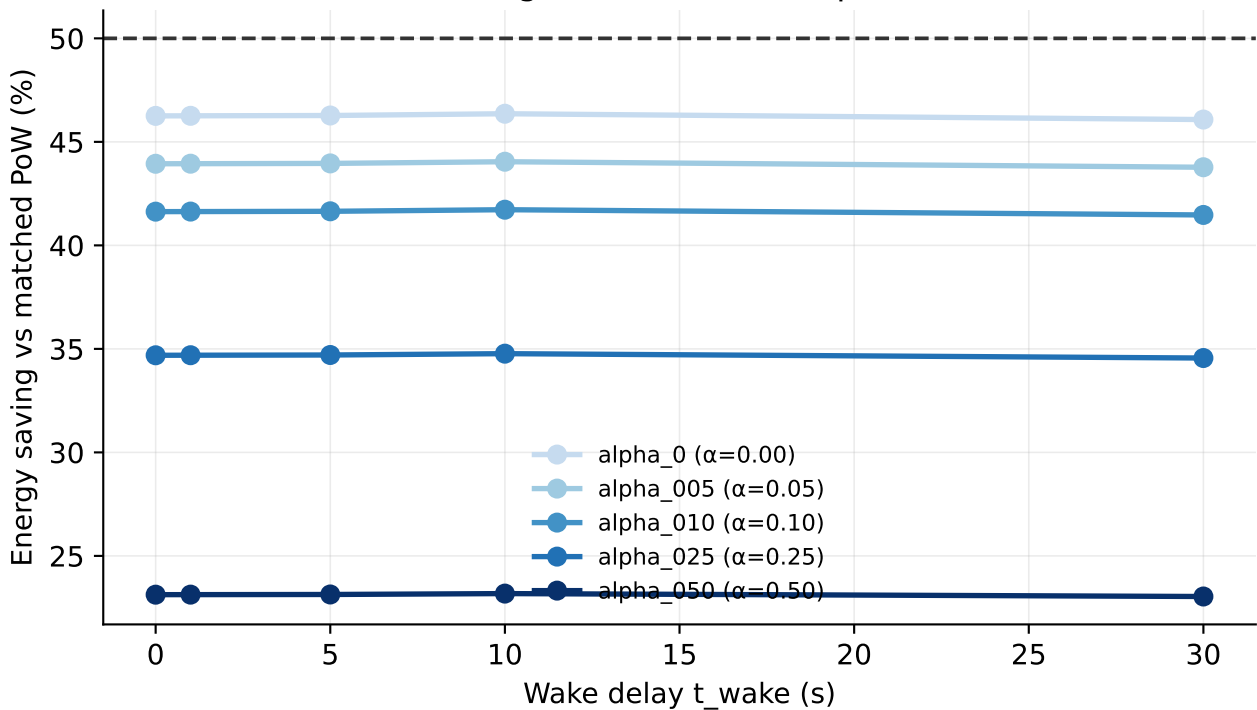
Energy saving vs wake delay (AdaptiveReserve, H2, N = 300) waking draws full active power
