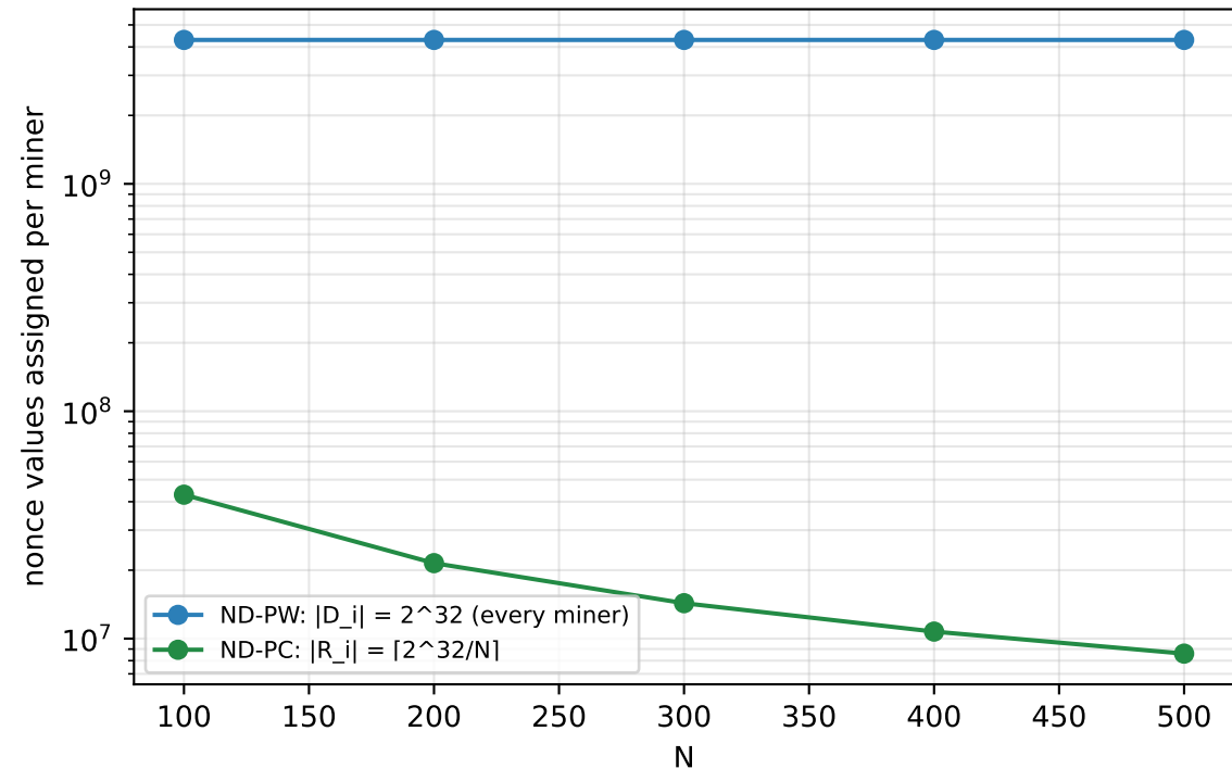
Same domain, different organization: full copy per PoW miner vs disjoint partition
