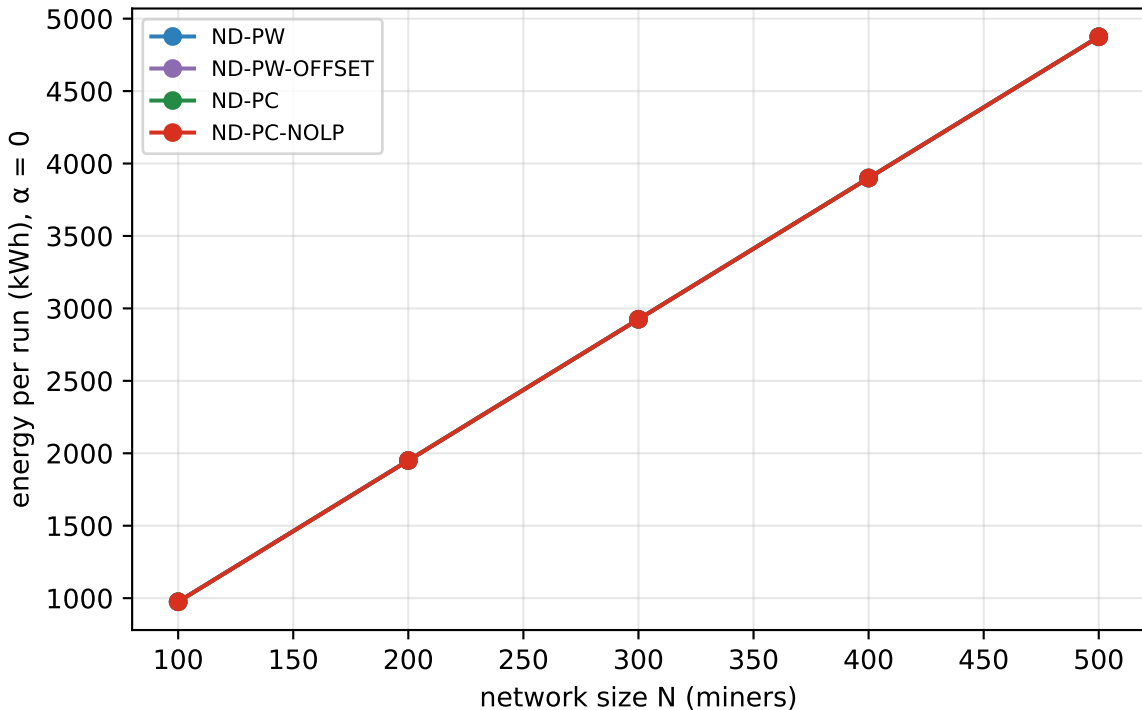
Total energy: all four arms coincide (differences \leq 7\text{e-}8 )
