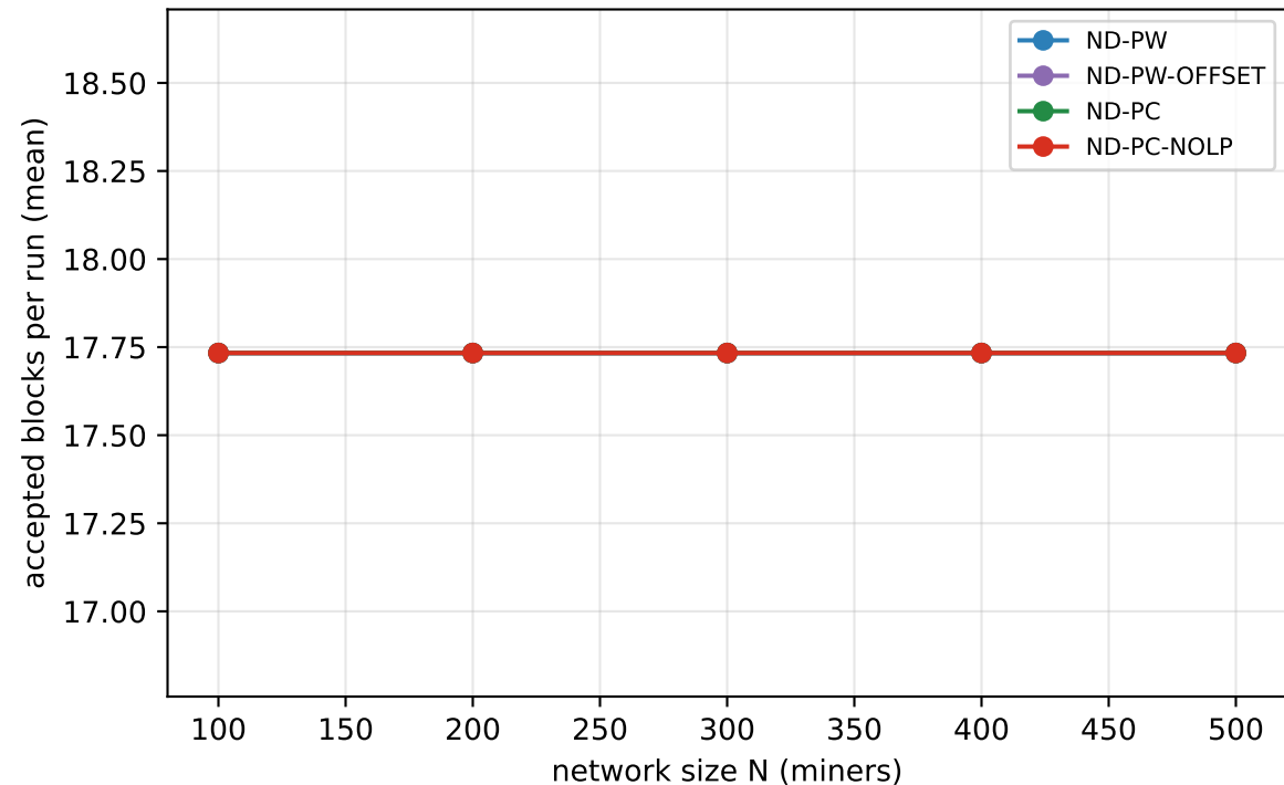
Block production identical: partitioning does not reduce independent trials per second (TQ4)
