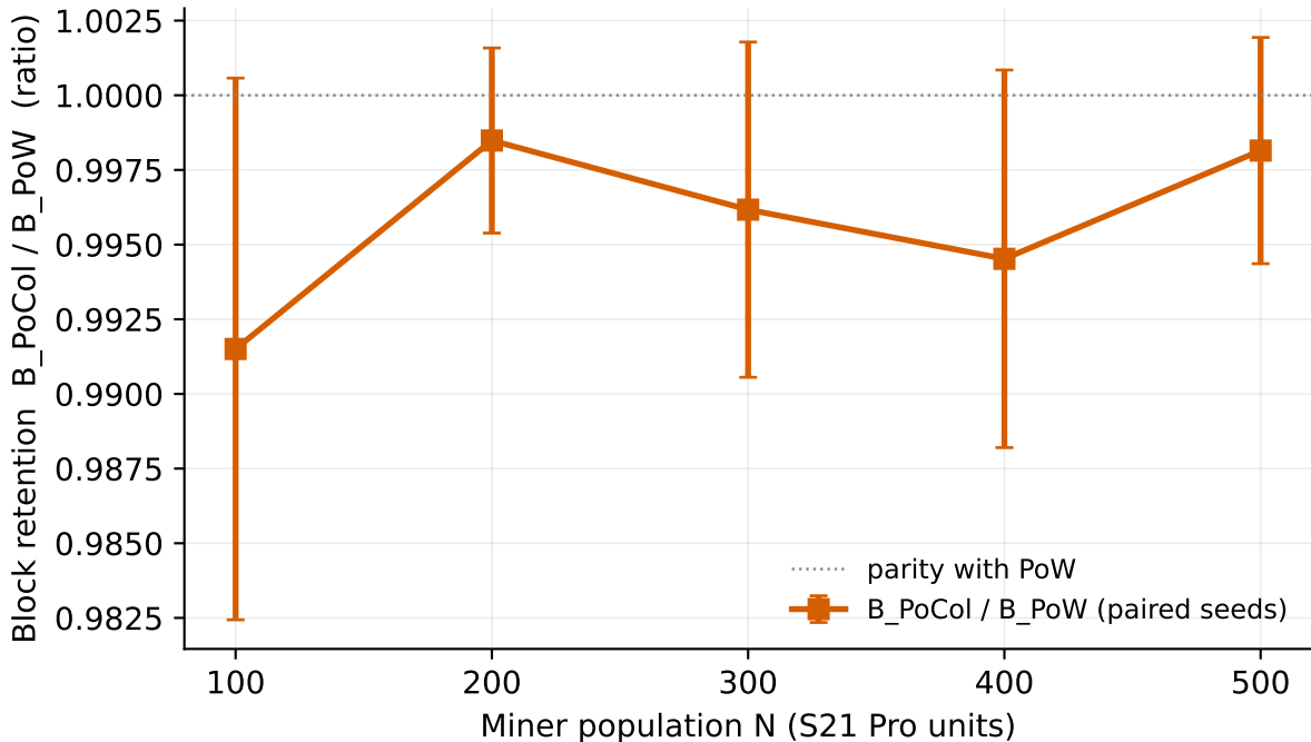
Block-retention ratio vs miner count (undefined pairs are dropped, never set to zero)
