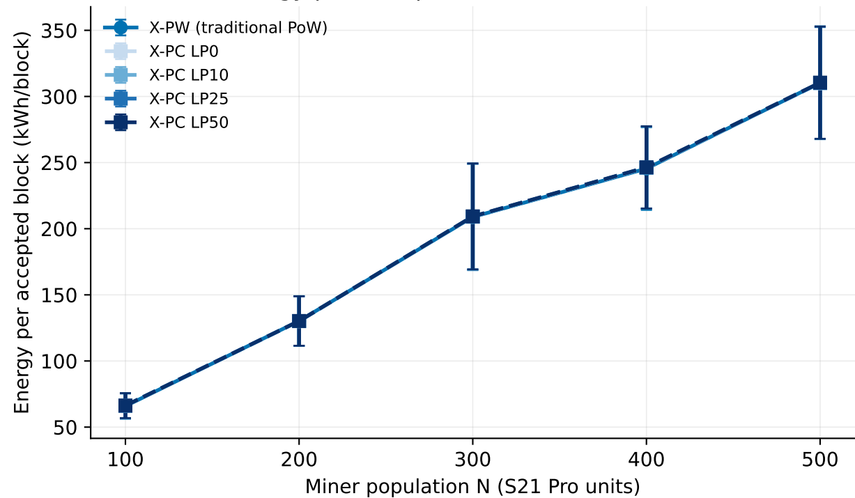
Energy per accepted block vs miner count
