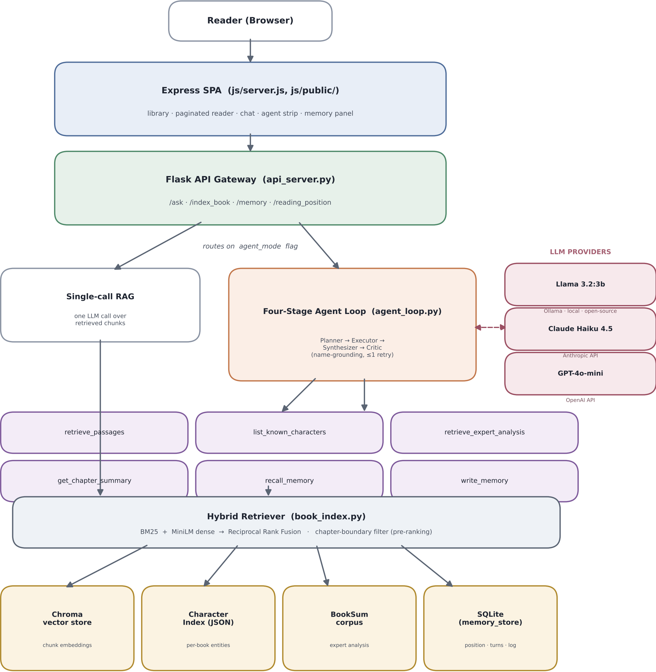
Figure 1. Literary Guide — System Architecture
