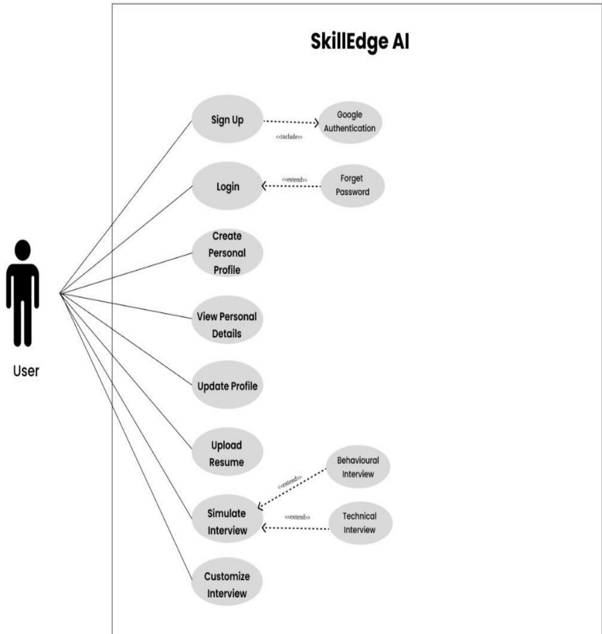
Figure 2: Use Case Diagram (1)
