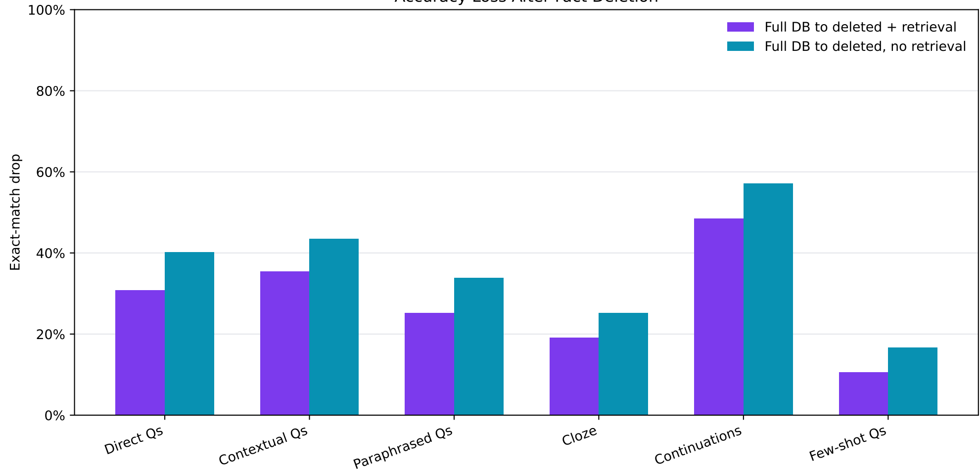
Accuracy Loss After Fact Deletion
